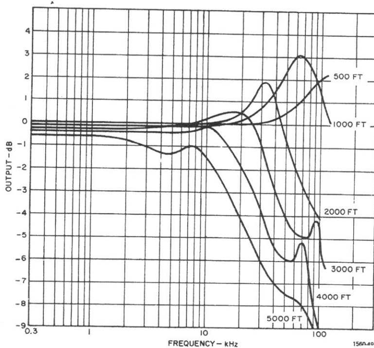
Figure 4-8. Measured cable loss of the Preamplifier vs cable length for Belden #8771 cable. Preamplifier gain is \times 1 , powered from the receiver end.
