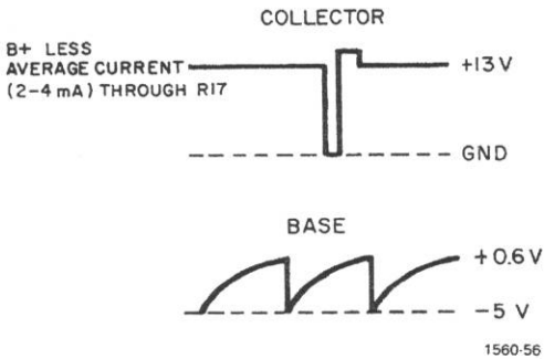
Figure 4-15. Waveforms at transistor Q5.
