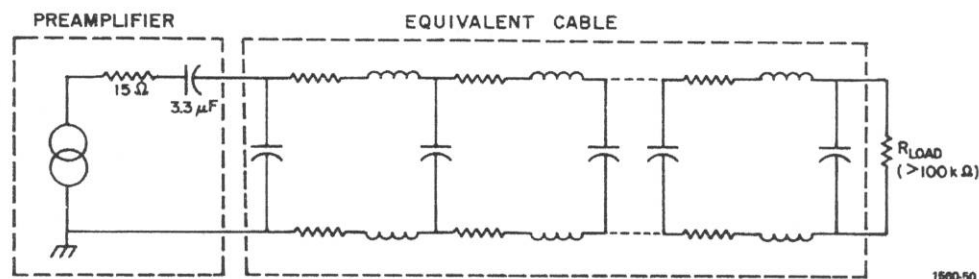
Figure 4-9. Equivalent circuit for long cables.
